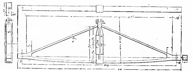
Figs. 1565-1567. Passenger Brake Beam, Westinghouse.
